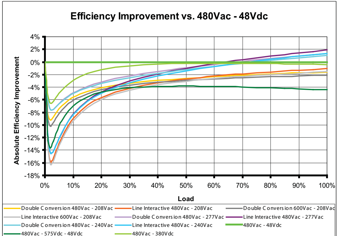
FIGURE 41. EFFICIENCY COMPARISON VS. 480VAC – 48VDC
