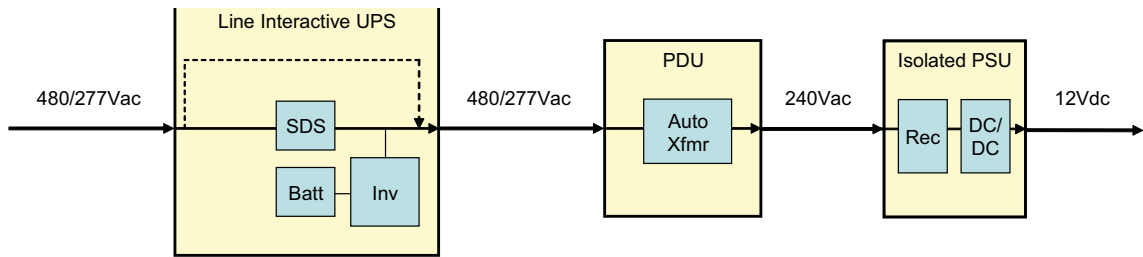
FIGURE 18. 480VAC – 240VAC CONFIGURATION WITH LINE INTERACTIVE UPS
