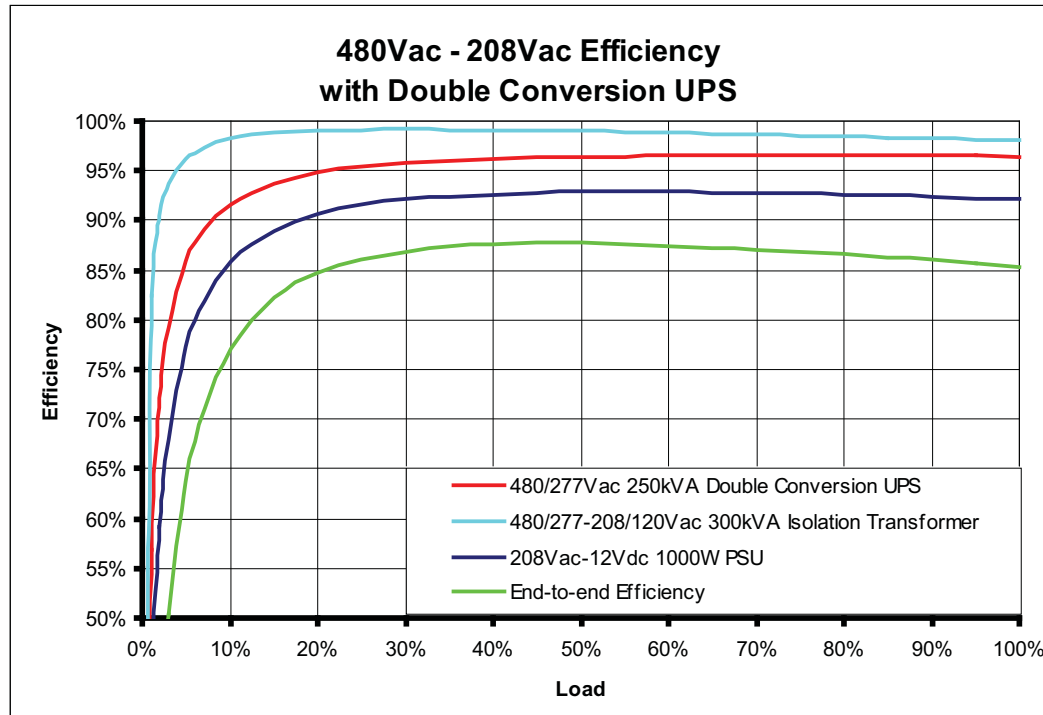
FIGURE 7. COMPONENT AND END-TO-END EFFICIENCY FOR 480VAC – 208VAC WITH DOUBLE CONVERSION UPS
