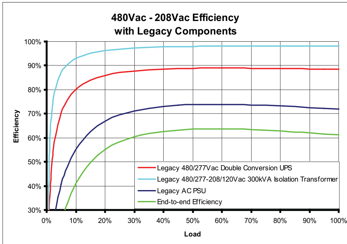
FIGURE 4. COMPONENT AND END-TO-END EFFICIENCY FOR LEGACY 480VAC – 208VAC CONFIGURATION
