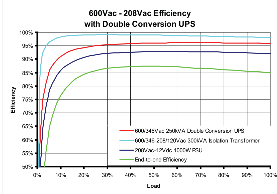
FIGURE 11. COMPONENT AND END-TO-END EFFICIENCY FOR 600VAC – 208VAC WITH DOUBLE CONVERSION UPS
