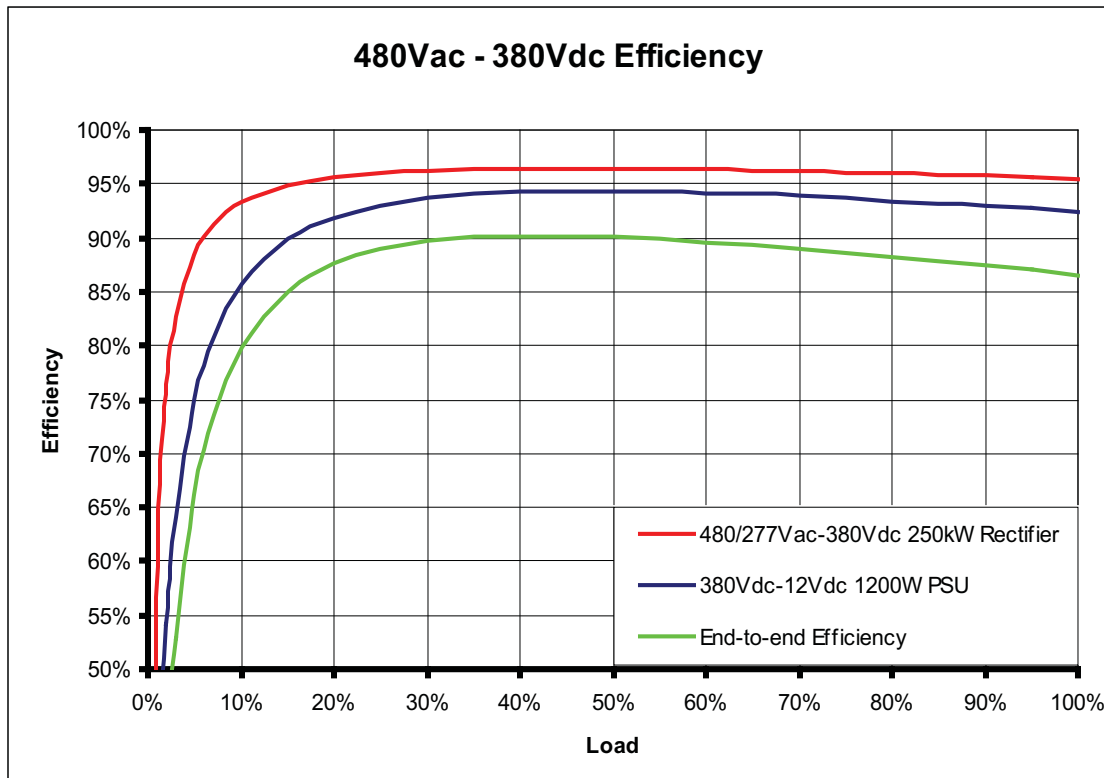
FIGURE 26. COMPONENT AND END-TO-END EFFICIENCY FOR 480VAC – 380VDC
