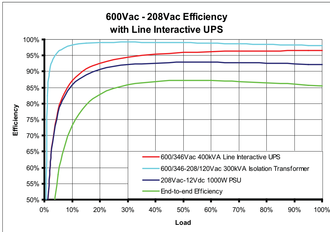
FIGURE 12. COMPONENT AND END-TO-END EFFICIENCY FOR 600VAC – 208VAC WITH LINE INTERACTIVE UPS
