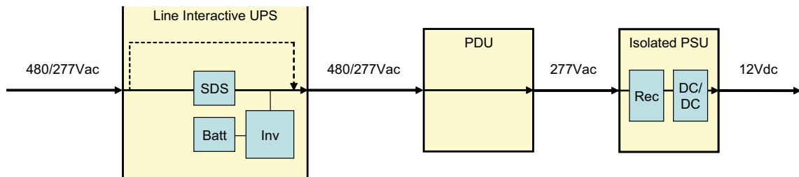
FIGURE 14. 480VAC – 277VAC CONFIGURATION WITH LINE INTERACTIVE UPS
