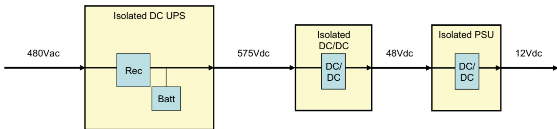
FIGURE 23. 480VAC – 575VDC – 48VDC CONFIGURATION
