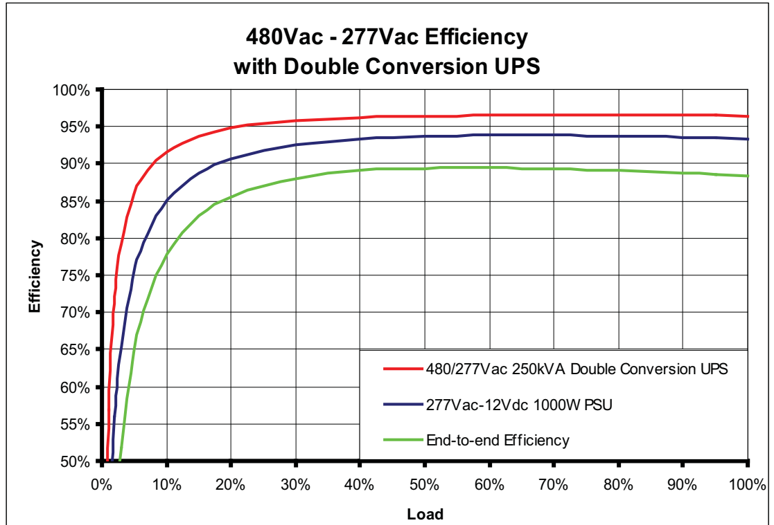
FIGURE 15. COMPONENT AND END-TO-END EFFICIENCY FOR 480VAC – 277VAC WITH DOUBLE CONVERSION UPS
