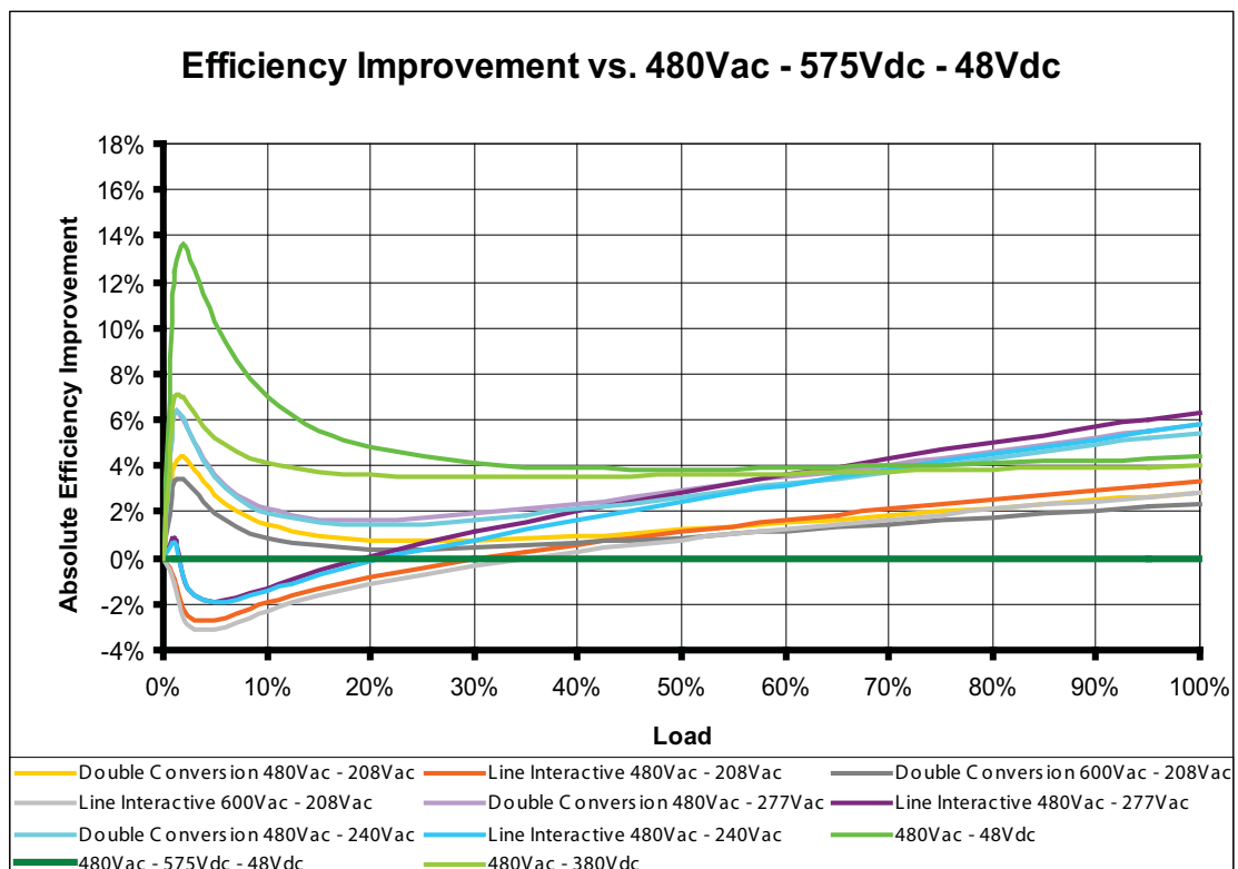
FIGURE 42. EFFICIENCY COMPARISON VS. 480VAC – 575VDC – 48VDC
